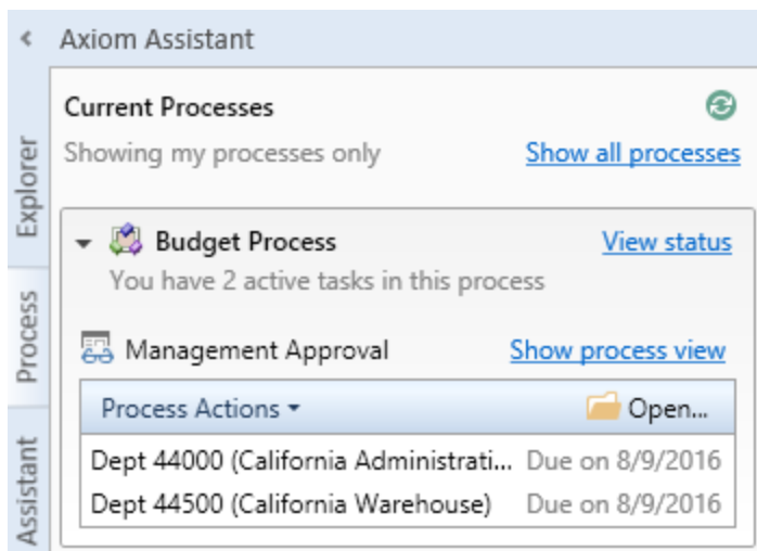
Example Process task pane with plan file tasks
